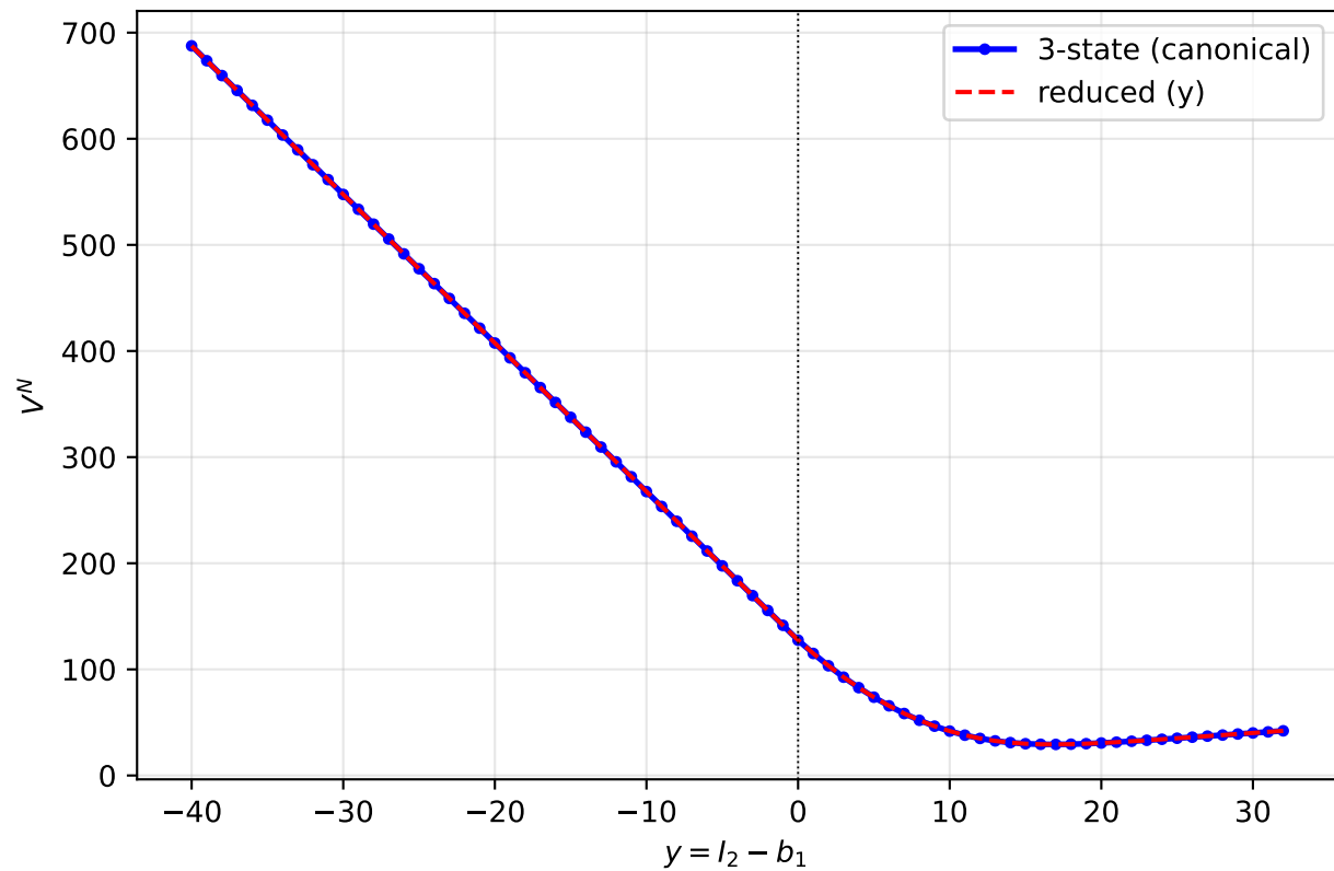
Value function (Run 1: exact)
